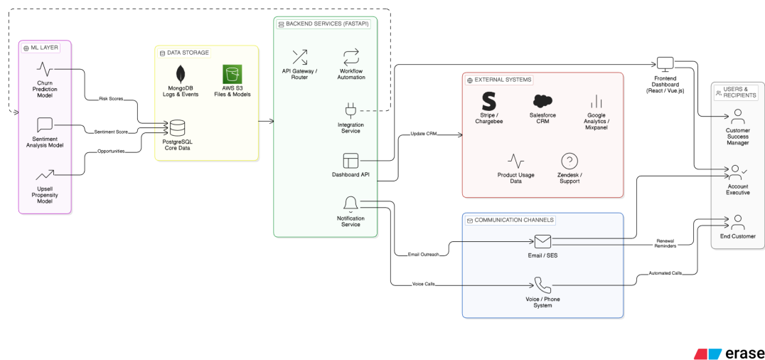
Figure 2: System Architecture Diagram - Detailed Data Flow
