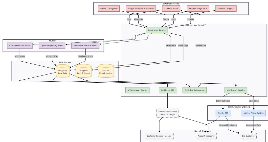
Figure 1: System Architecture Diagram - High Level
